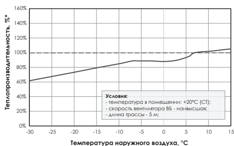
RCI-FHE75HN/OUT
