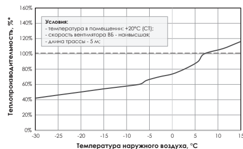
RCI-FHE55HN/OUT
