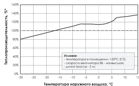
RCI-FHE55HN/OUT
